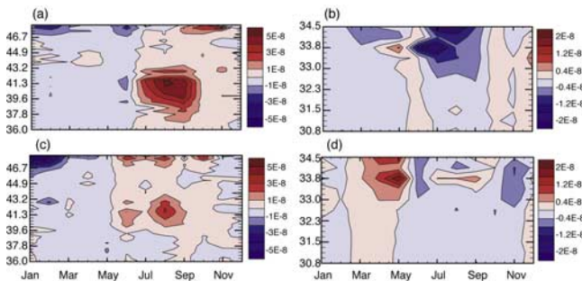
Figure 3. Latitude-Time plot showing the difference of zonally averaged wind-stress curl. (a) Northern region difference of 2X-1X, (b) Central region difference of 2X-1X, (c) Northern region difference of FUTURE-MODERN, (d) Central region difference of FUTURE-MODERN.
